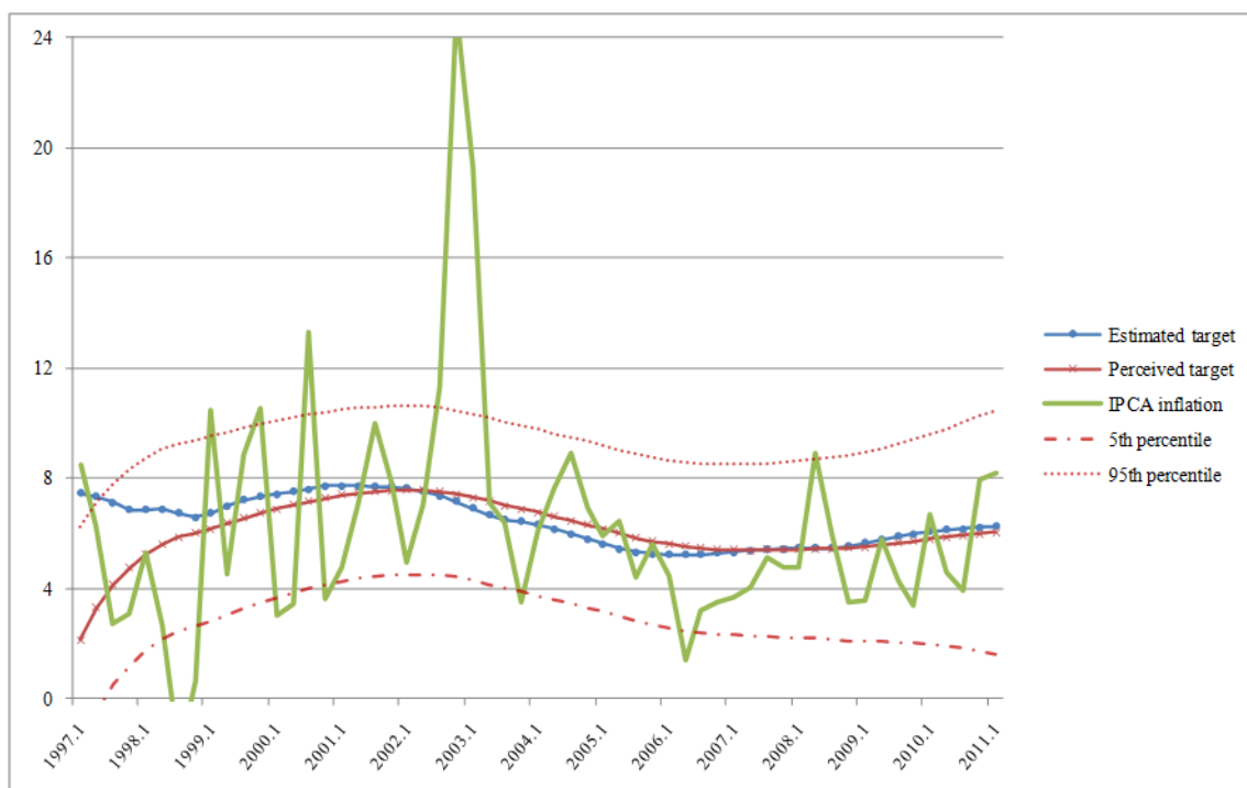
Figure 2: Unobserved targets and inflation (yearly %) - Multivariate model
