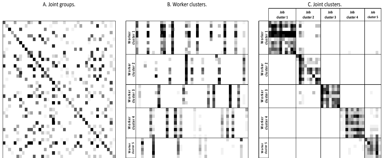
Fig. 4. Clustering process.
